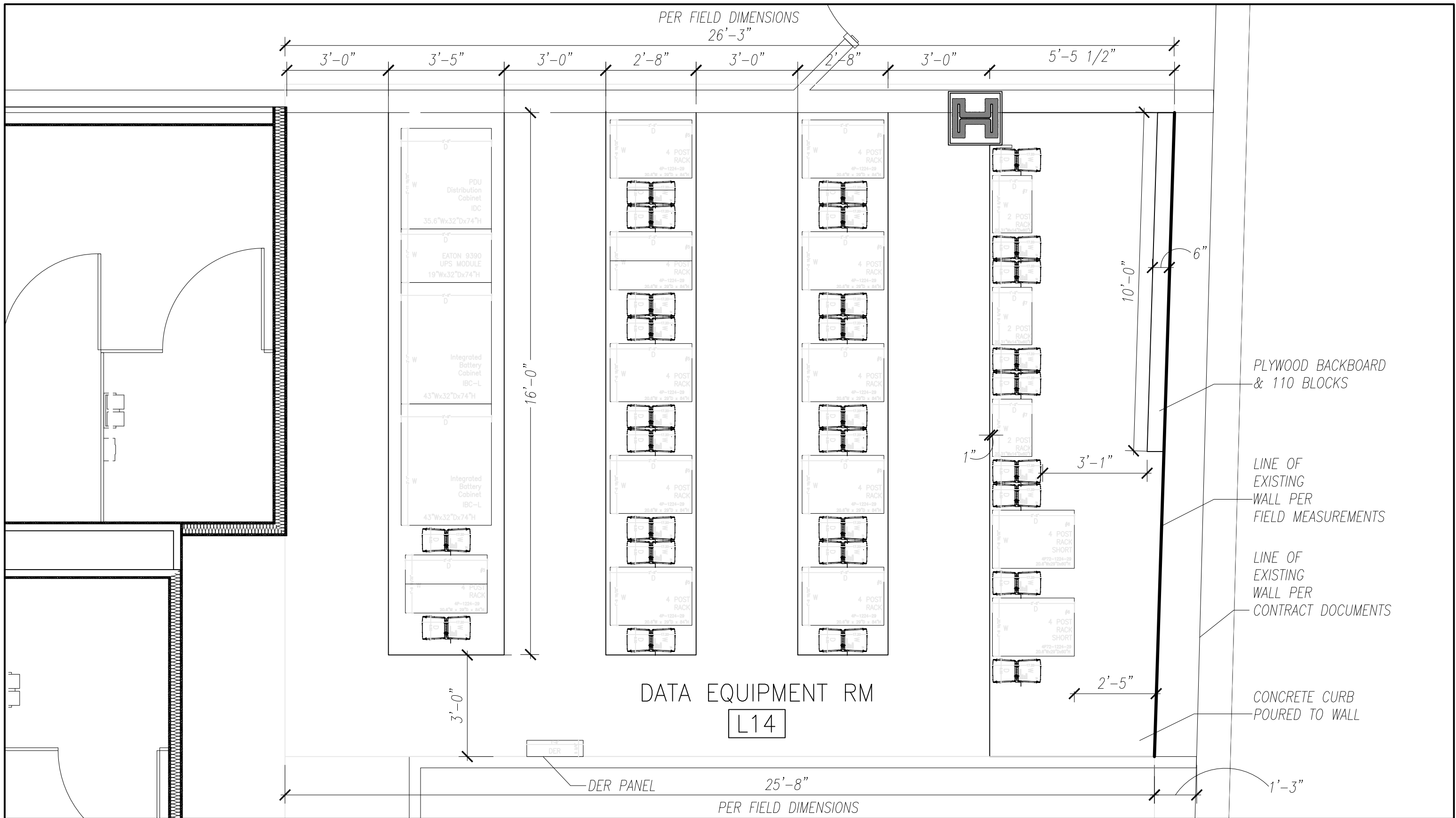
L14 DATA ROOM LAYOUT
