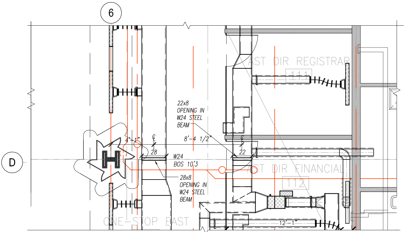
Location of Steel Penetrations
