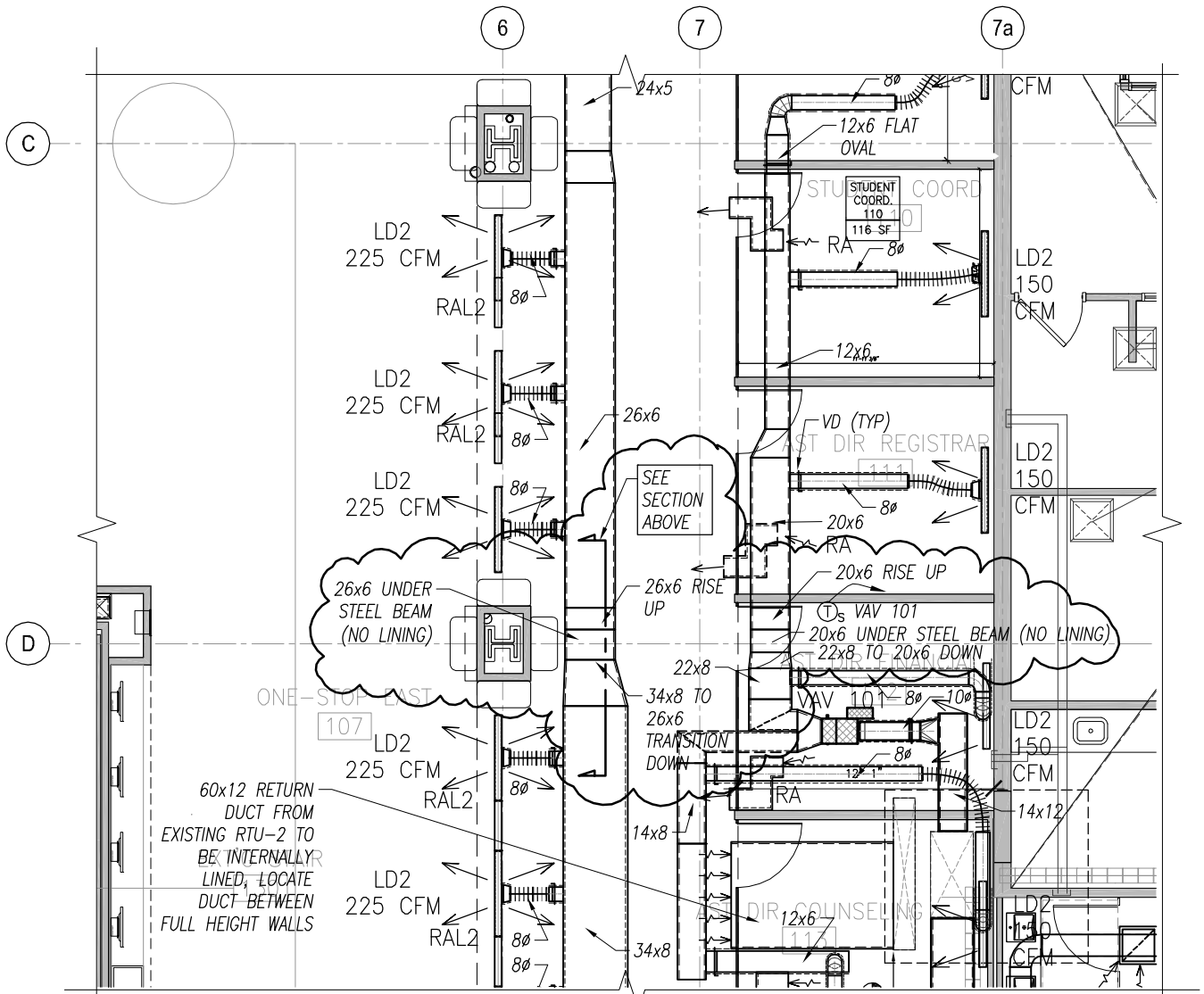
DUCTWORK UNDER STEEL BEAM AT COL C6 CLARIFICATION
