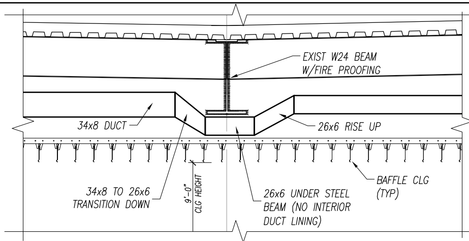
DUCT SECTION AT COL "D"
