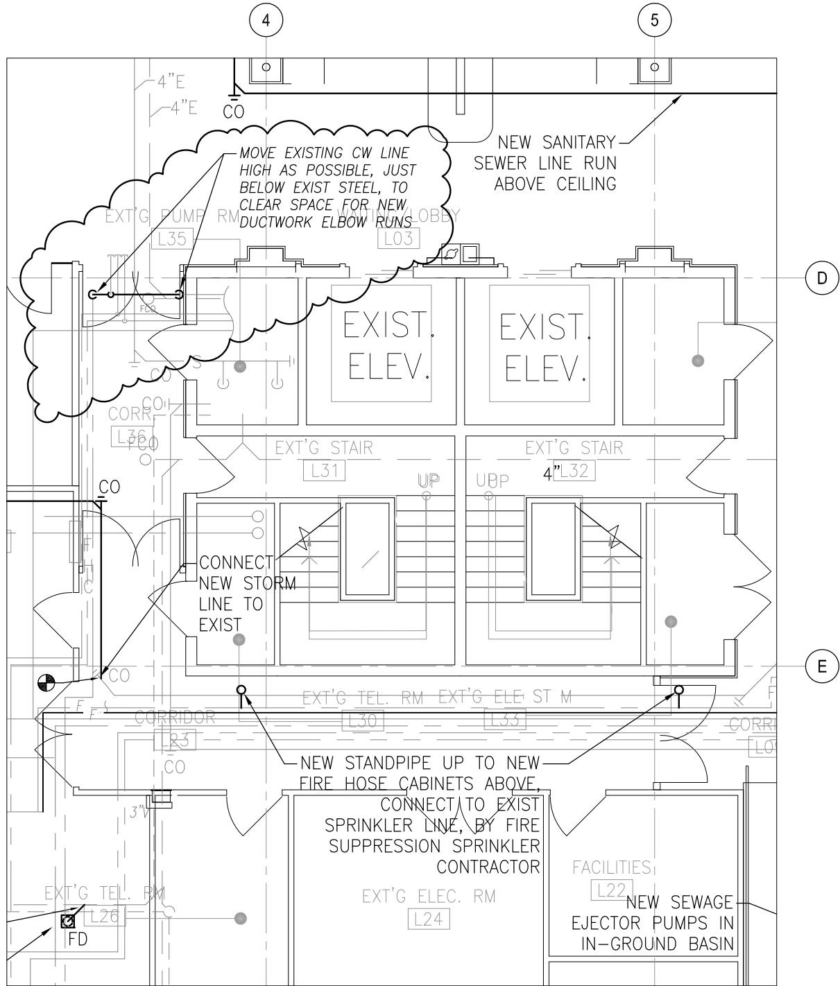
RELOCATION OF EXISTING COLD WATER LINE
