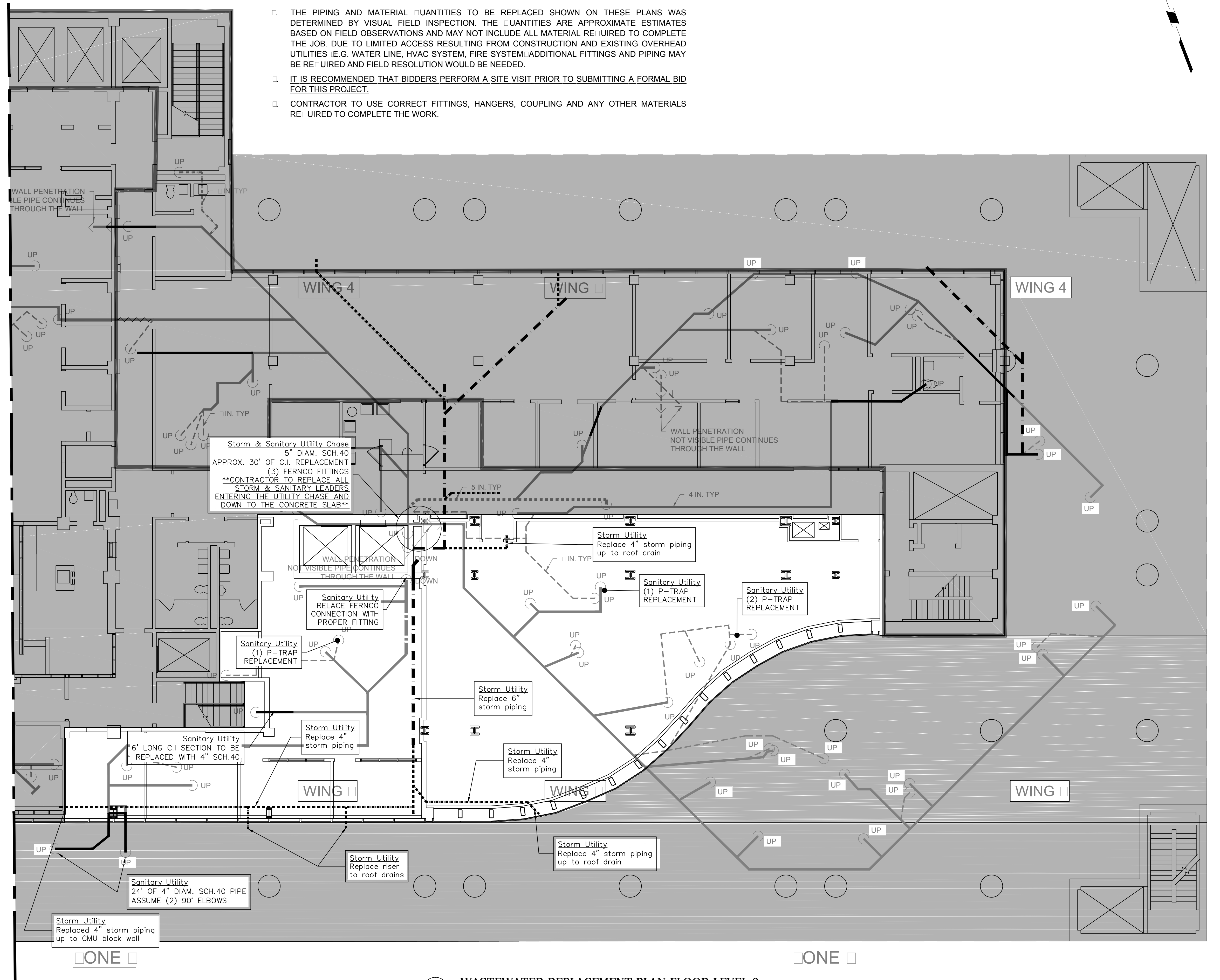
1 WASTEWATER REPLACEMENT PLAN FLOOR LEVEL 3 SCALE: 1/8"=1'-0"
