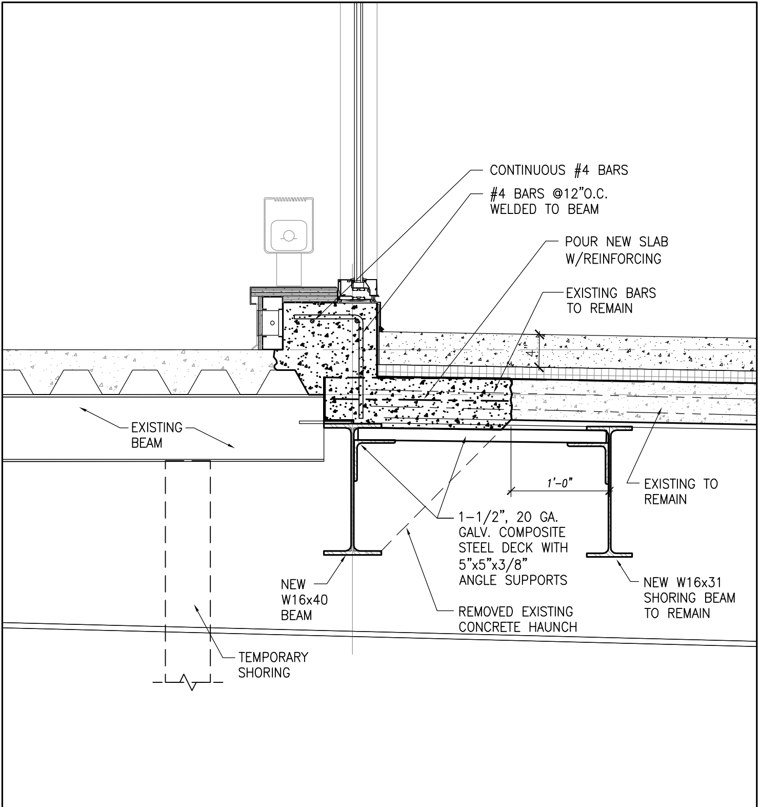
ALTERNATE DETERIORATED BEAM RECONSTRUCTION DETAIL
