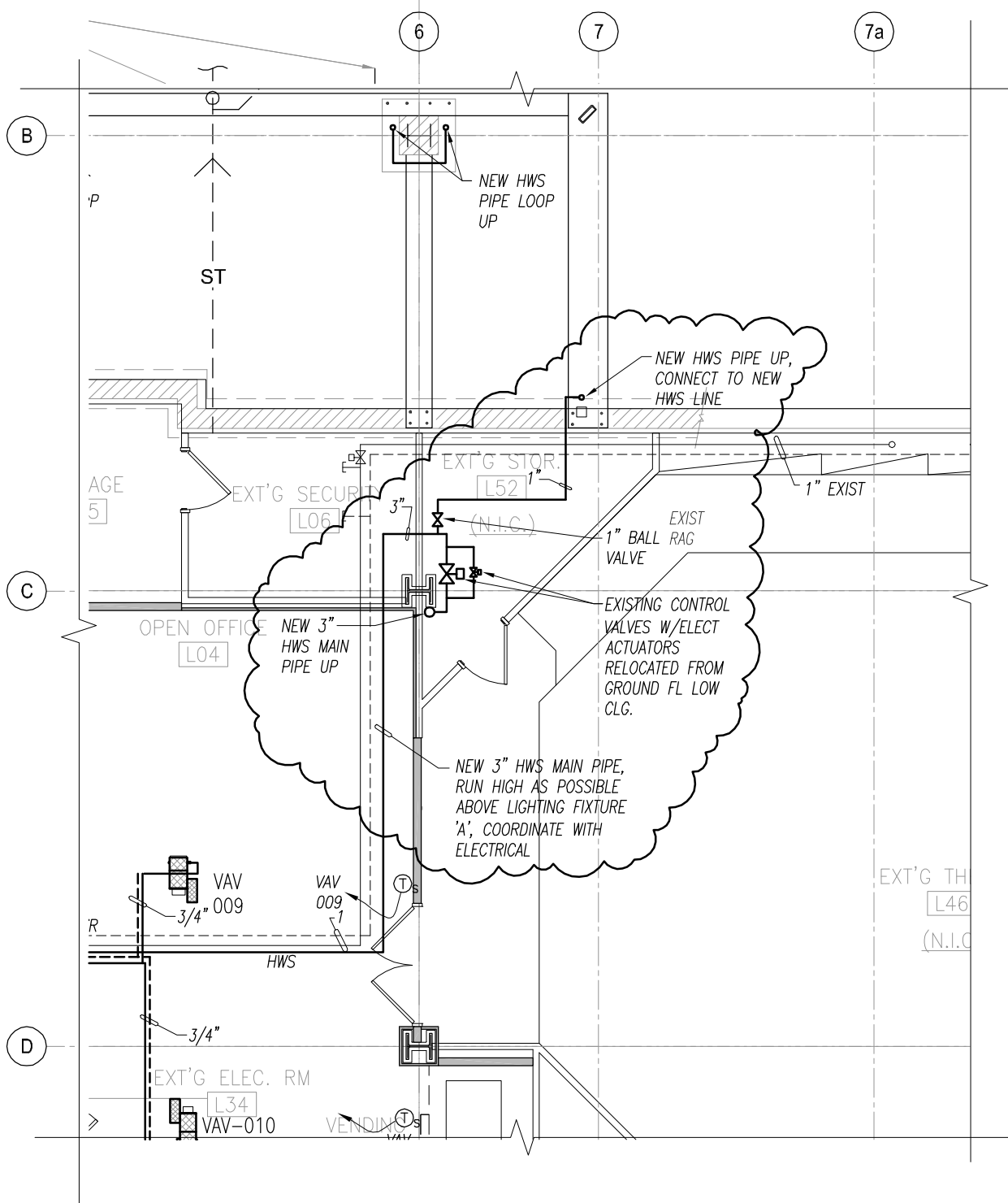
HOT WATER SUPPLY ROUTING SKETCH LOWER LEVEL PLAN SCALE: 1/8" = 1'-0"
