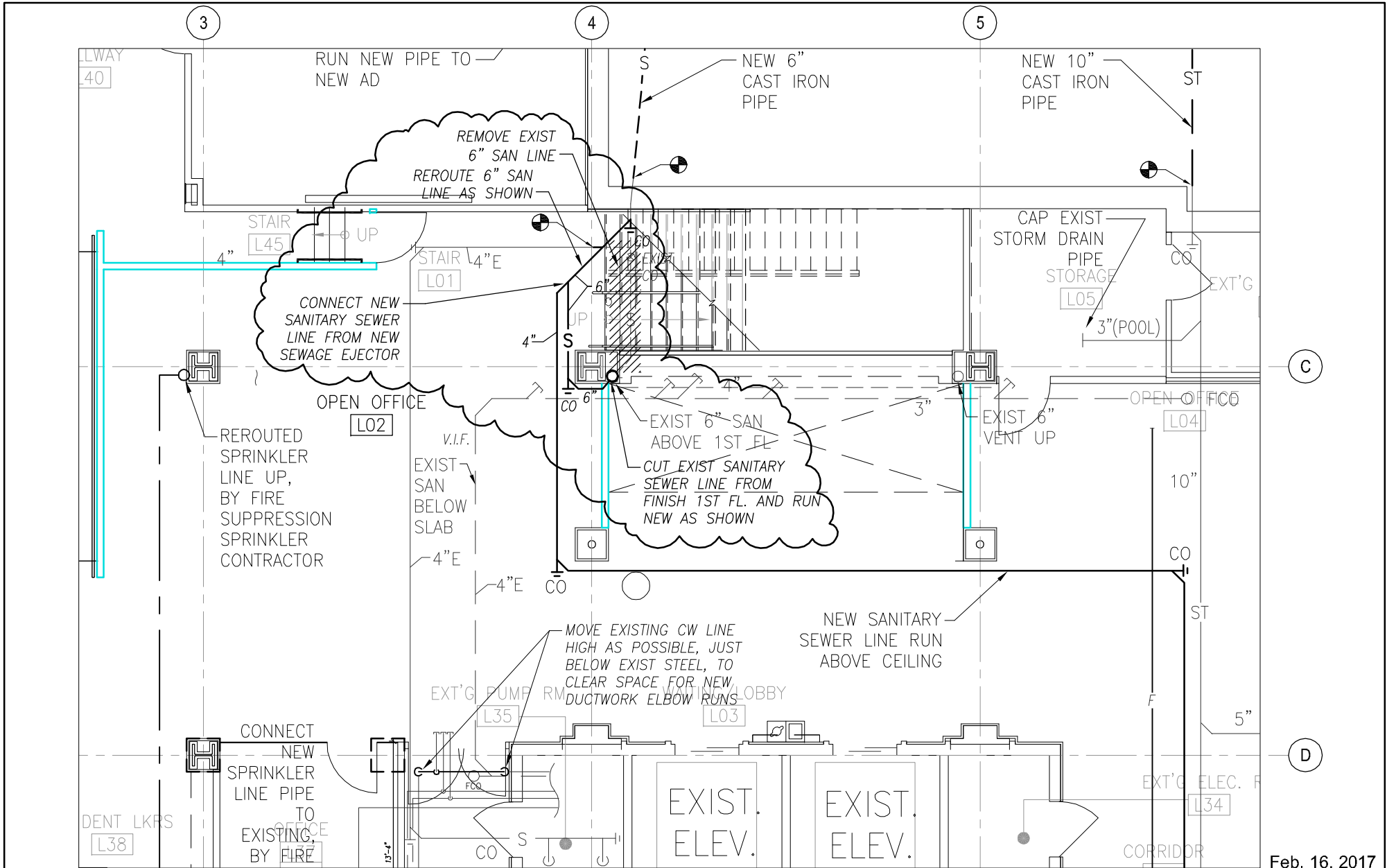
1 Partial Lower Level Plan SCALE: 1/8" = 1'-0"
