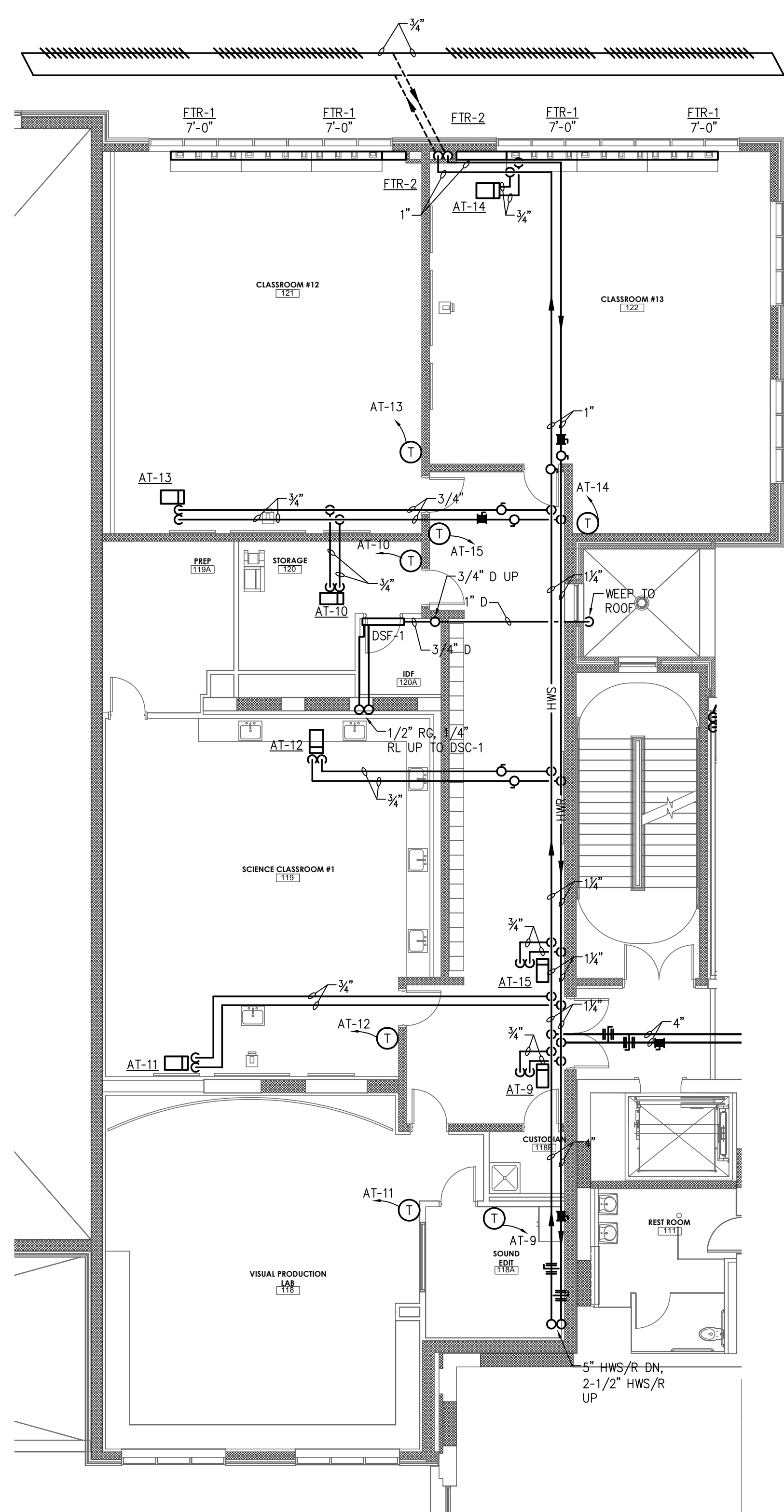
1 HVAC FIRST FLOOR PIPING PLAN H2.04 1/8" = 1'-0"
