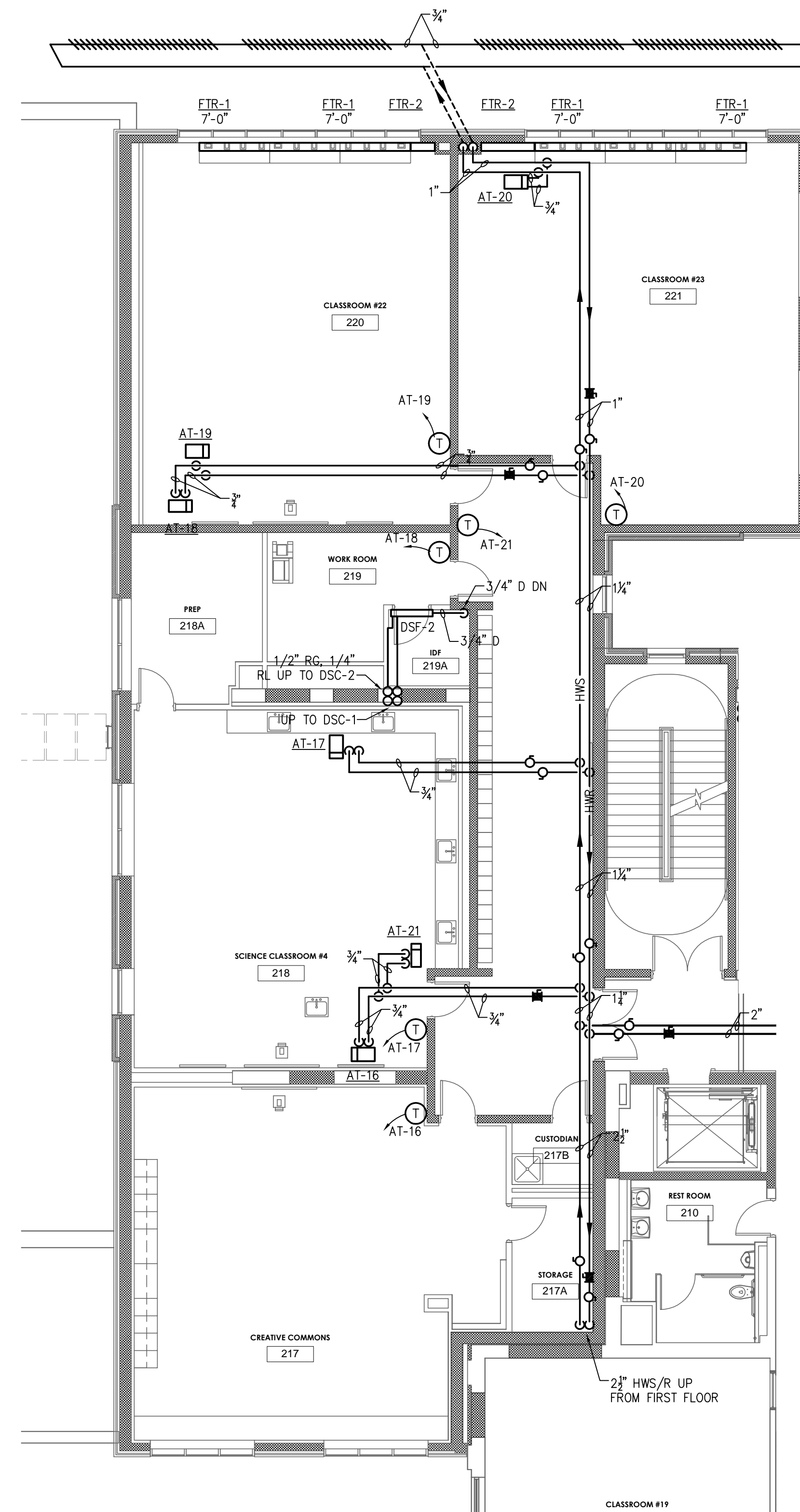
2 HVAC SECOND FLOOR PIPING PLAN H2.04 1/8" = 1'-0"
