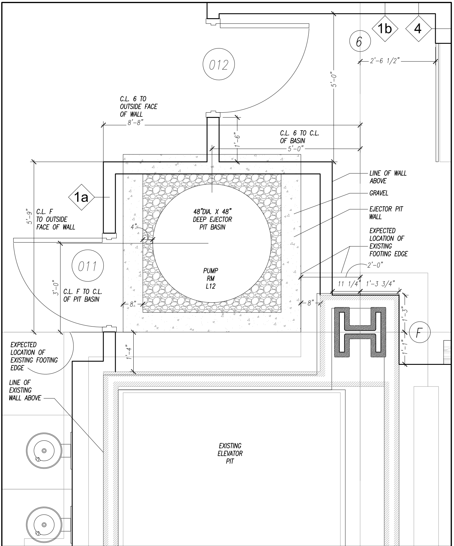
EJECTOR PIT FOUNDATION PLAN
