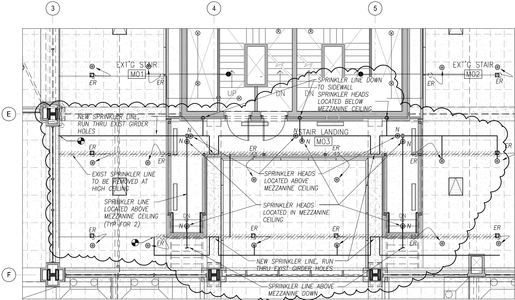
FP-103 Part First Floor Upper Level Sprinkler Mezzanine Layout
