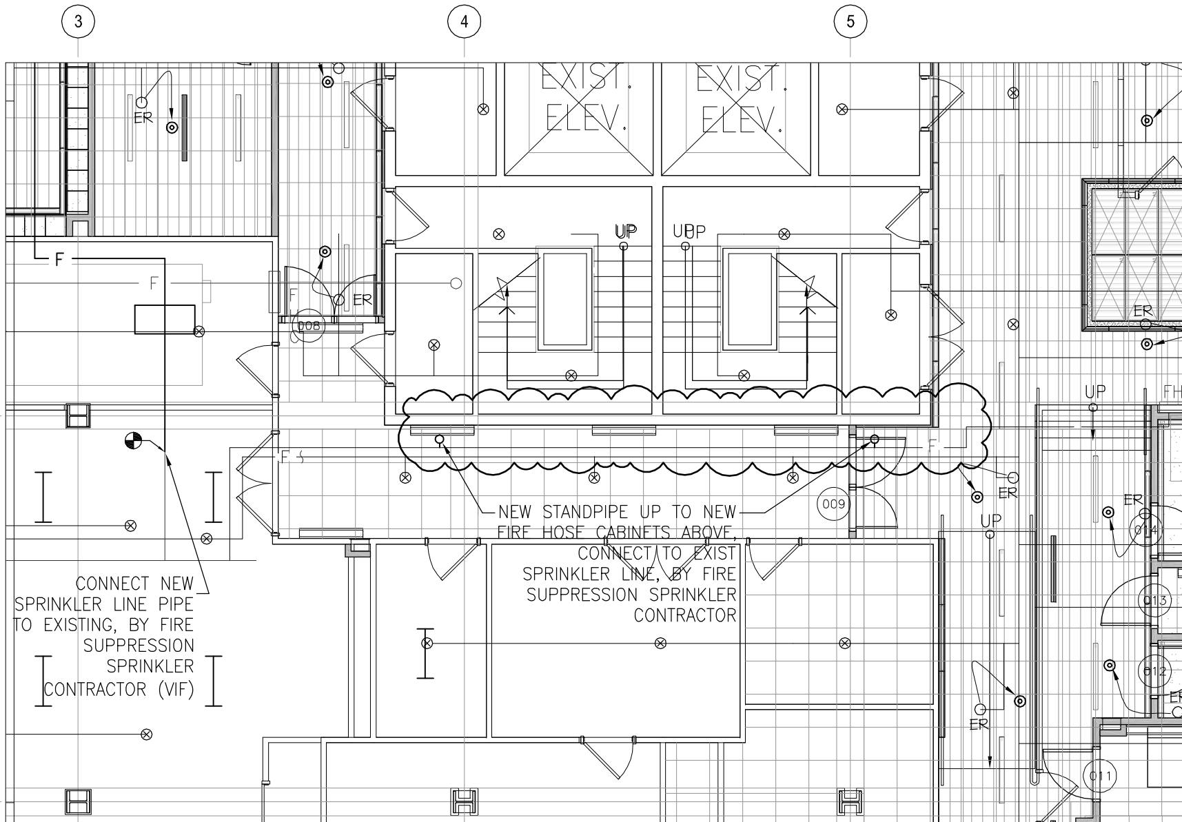
FP-101 Part Lower Level Sprinkler Layout
