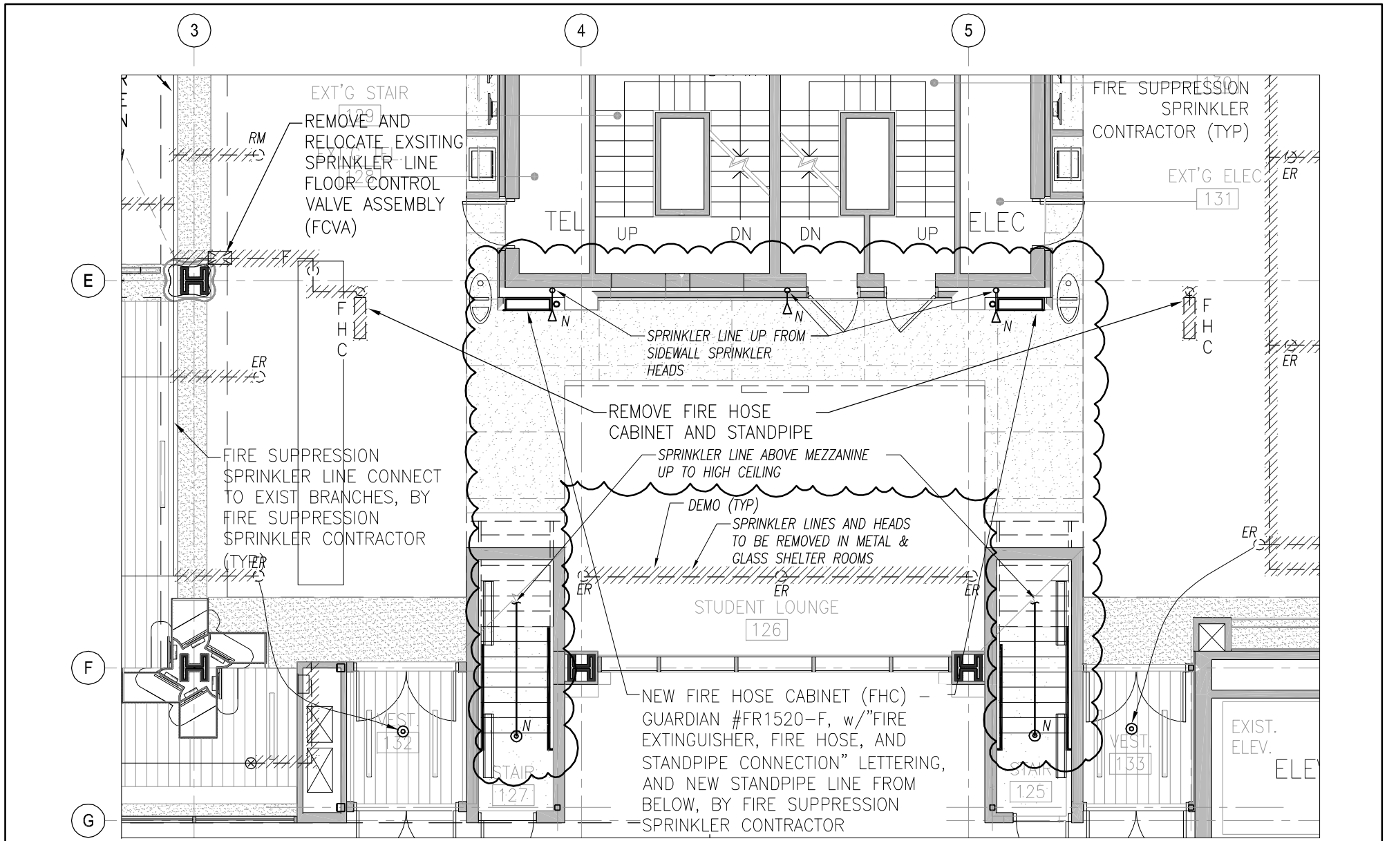
FP-102 Part First Floor Low Level Sprinkler Layout
