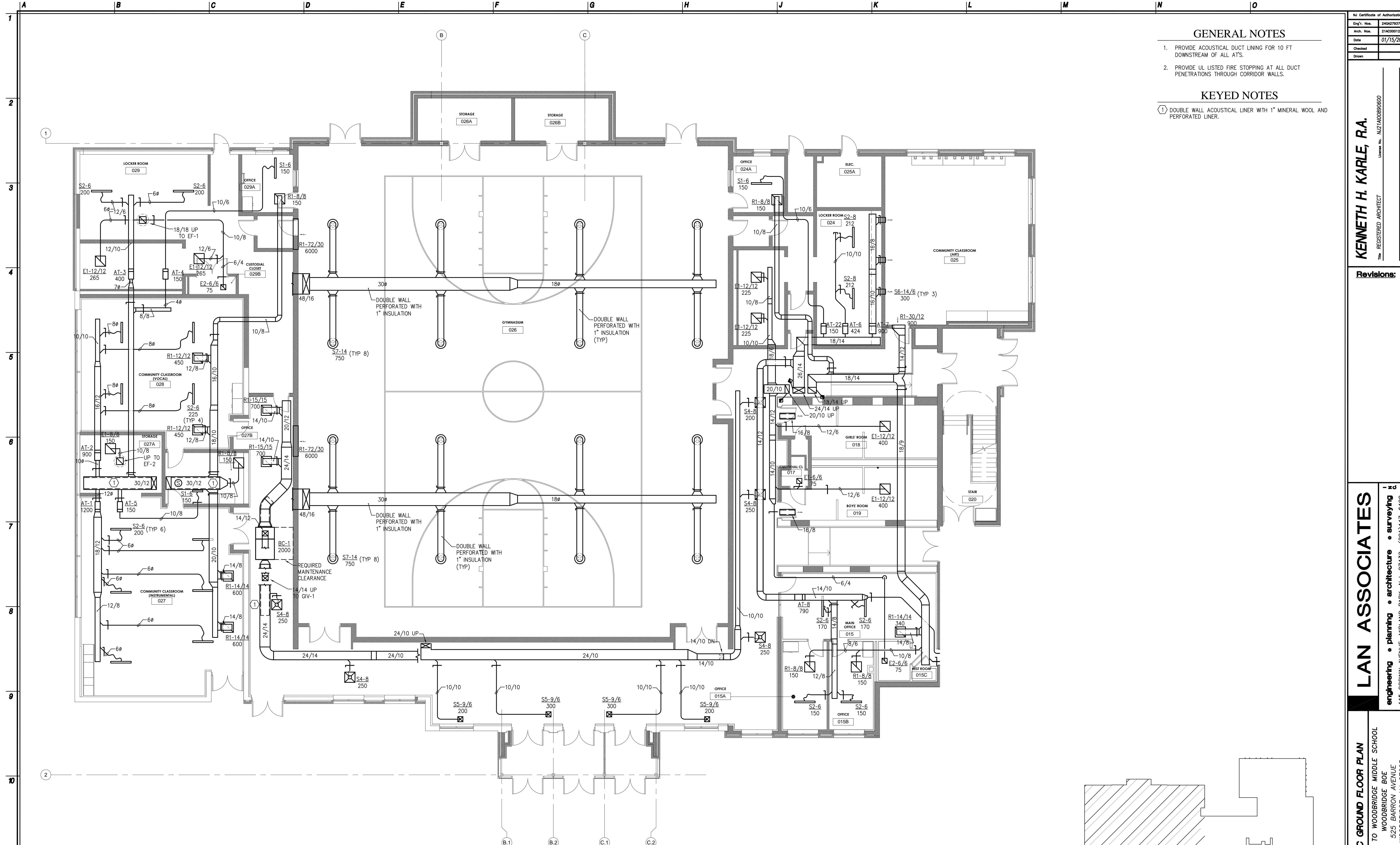
1 HVAC GROUND FLOOR PLAN H1.01 1/8" = 1'-0"
