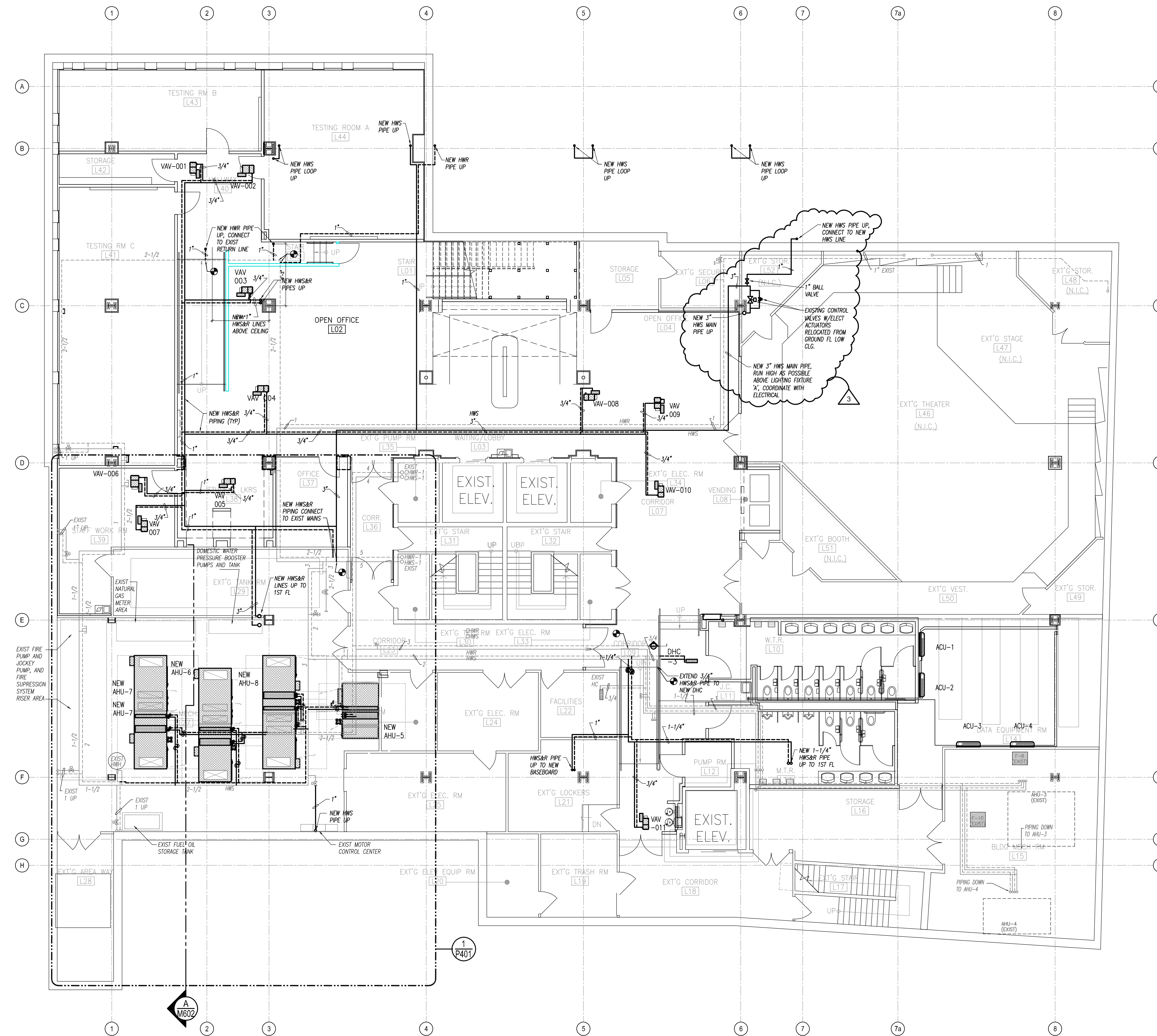
PIPING LOWER LEVEL PLAN SCALE: 1/8" = 1'-0"
