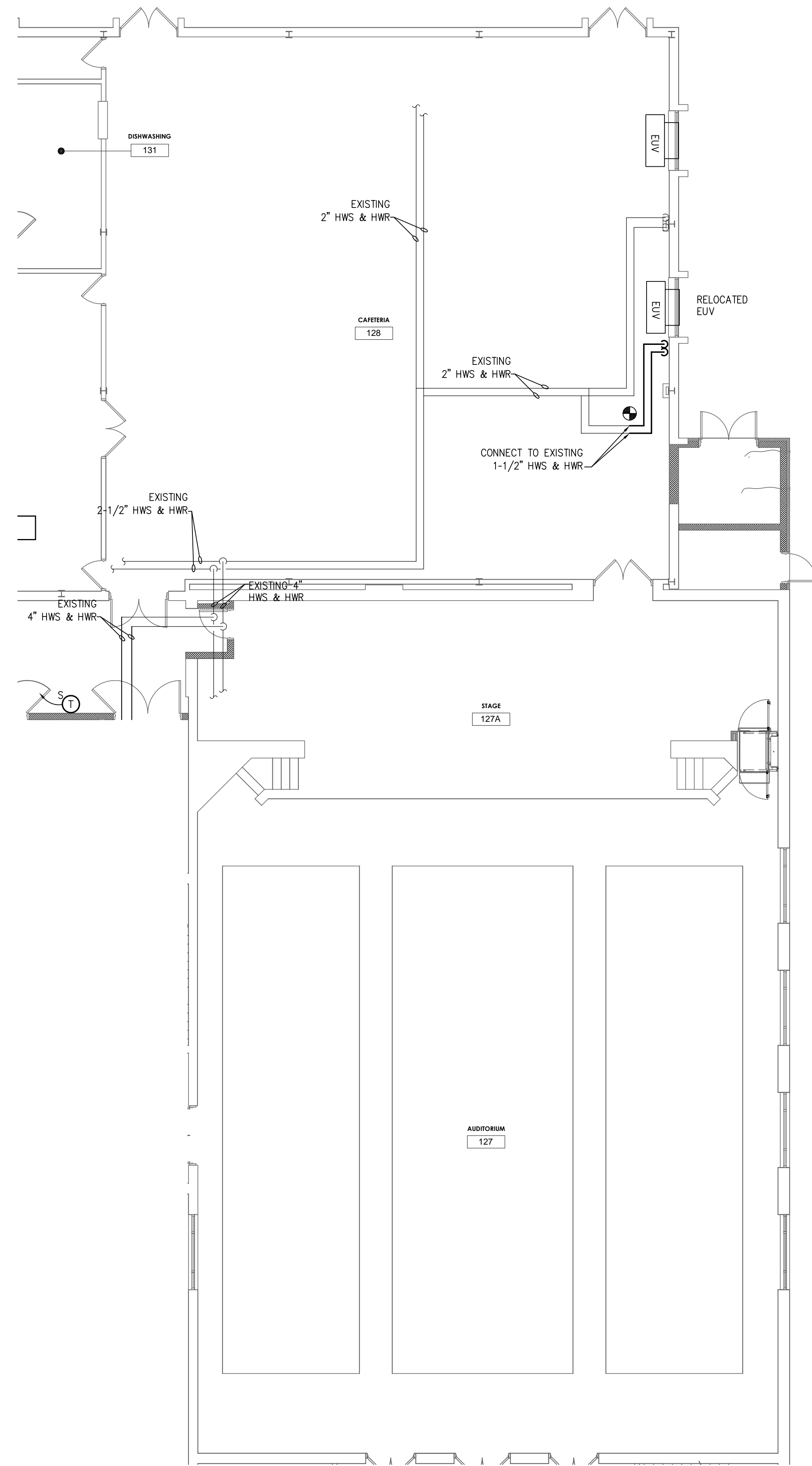
1 H2.03 HVAC GROUND FLOOR PIPING PLAN *****
