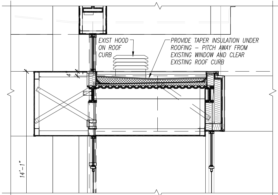
Section A-A at Col F-6 Near Existing Elevator
