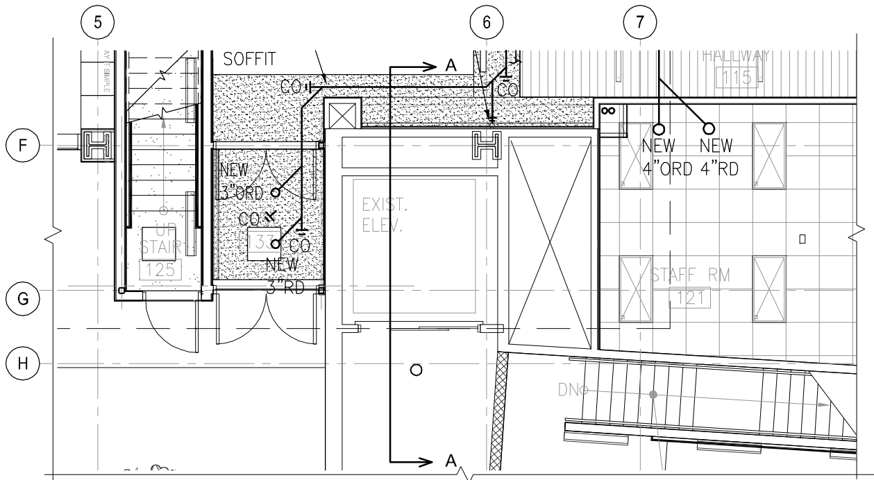
Location and Routing of New 3" Roof Drains Over Existing Elevator
