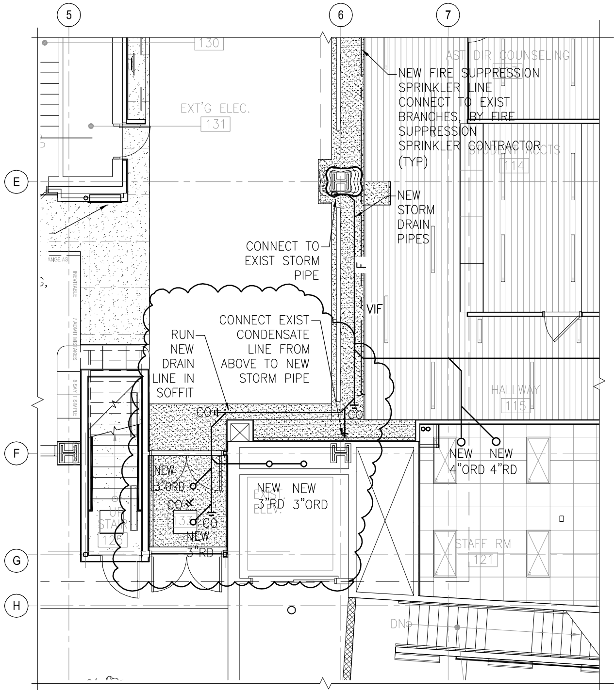
Location and Routing of New 3" Roof Drains Over Existing Elevator
