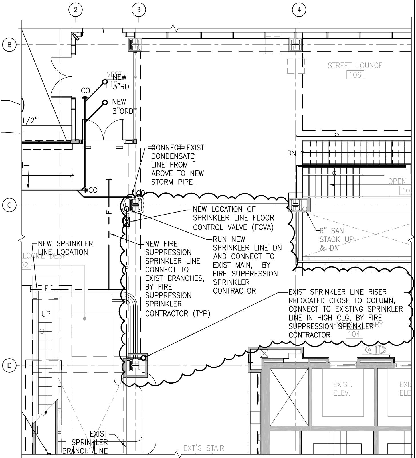
Location of Sprinkler Line Floor Control Valve Assembly
