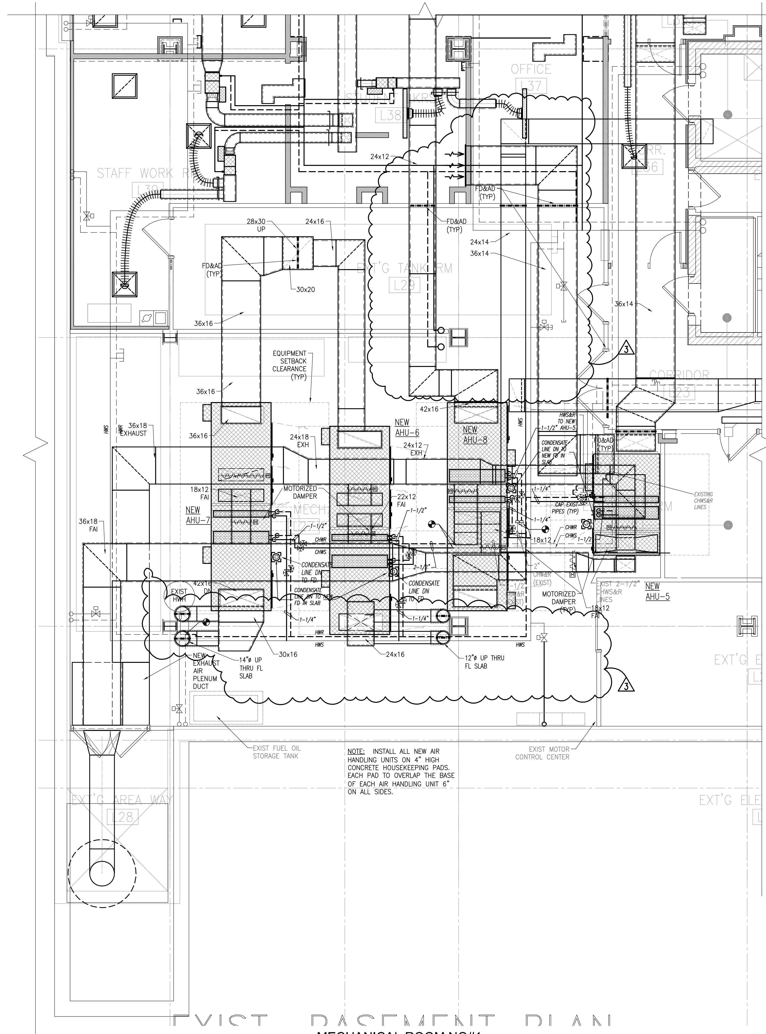
MECHANICAL ROOM NO#1 ENLARGED LOWER LEVEL PLAN SCALE: 1/4" = 1'-0"
