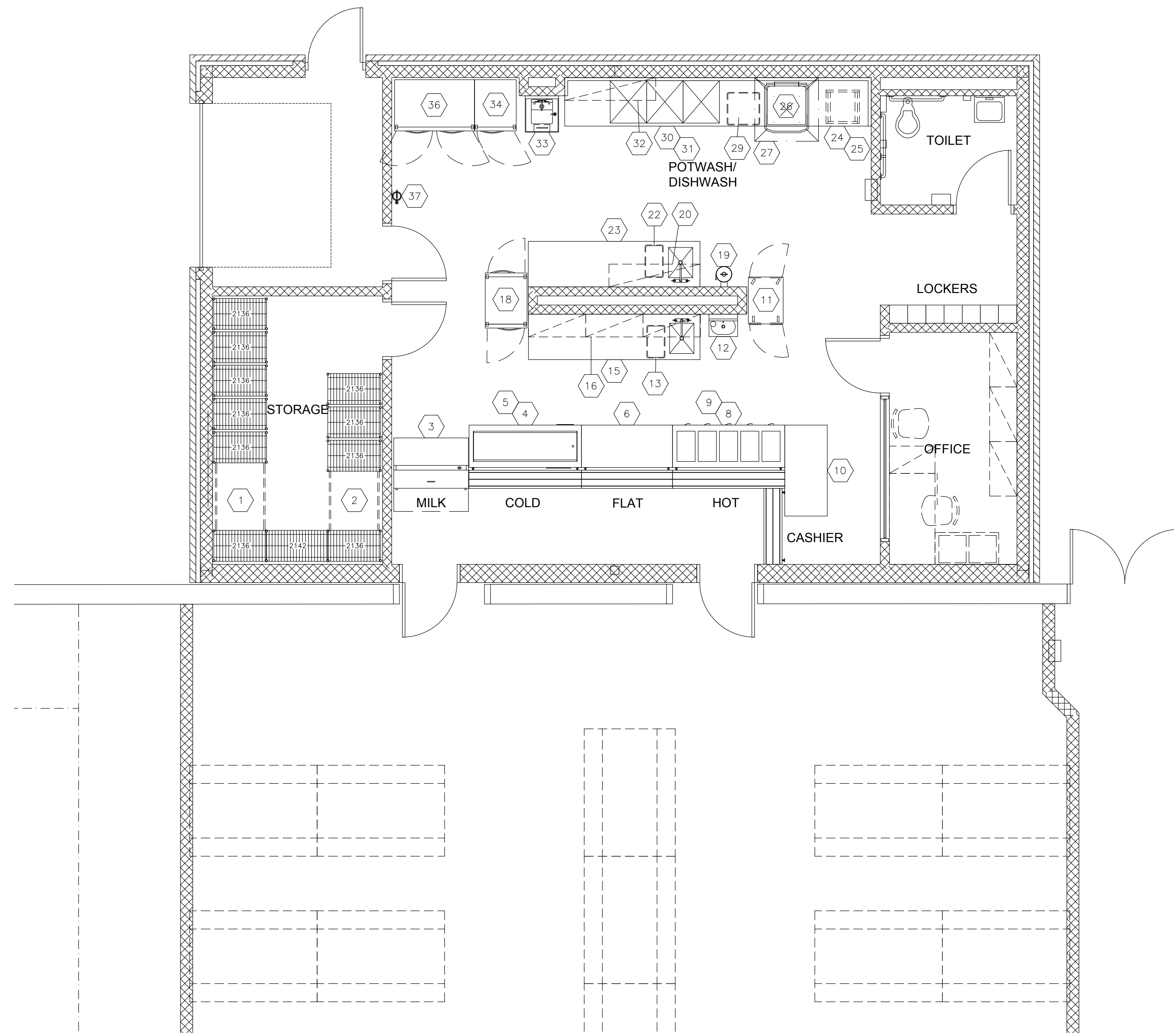
FOOD SERVICE EQUIPMENT PLAN SCALE: 1/4"=1'-0"
