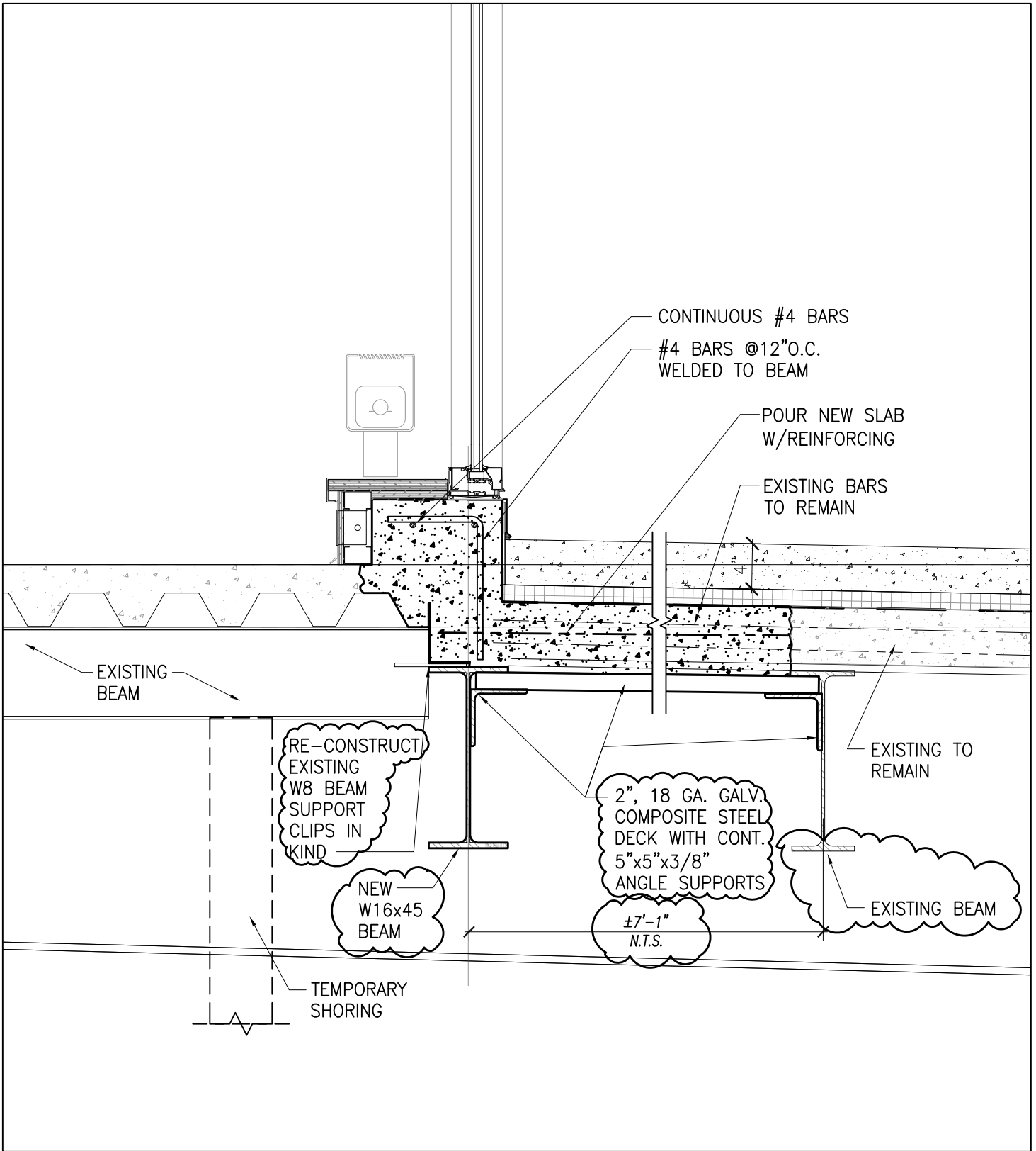
ALTERNATE DETERIORATED BEAM RECONSTRUCTION DETAIL
