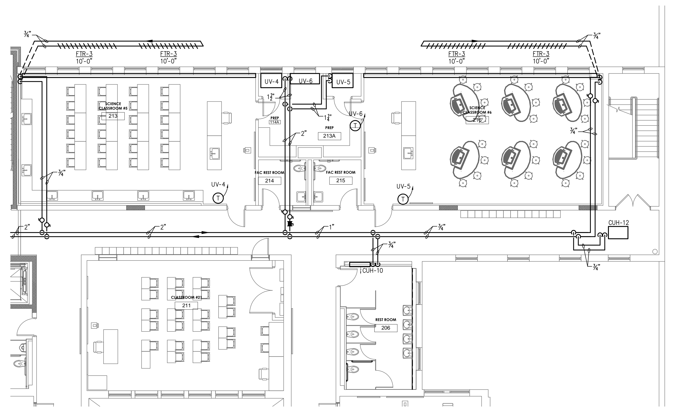
2 HVAC SECOND FLOOR PIPING PLAN H2.05 1/8" = 1'-0"
