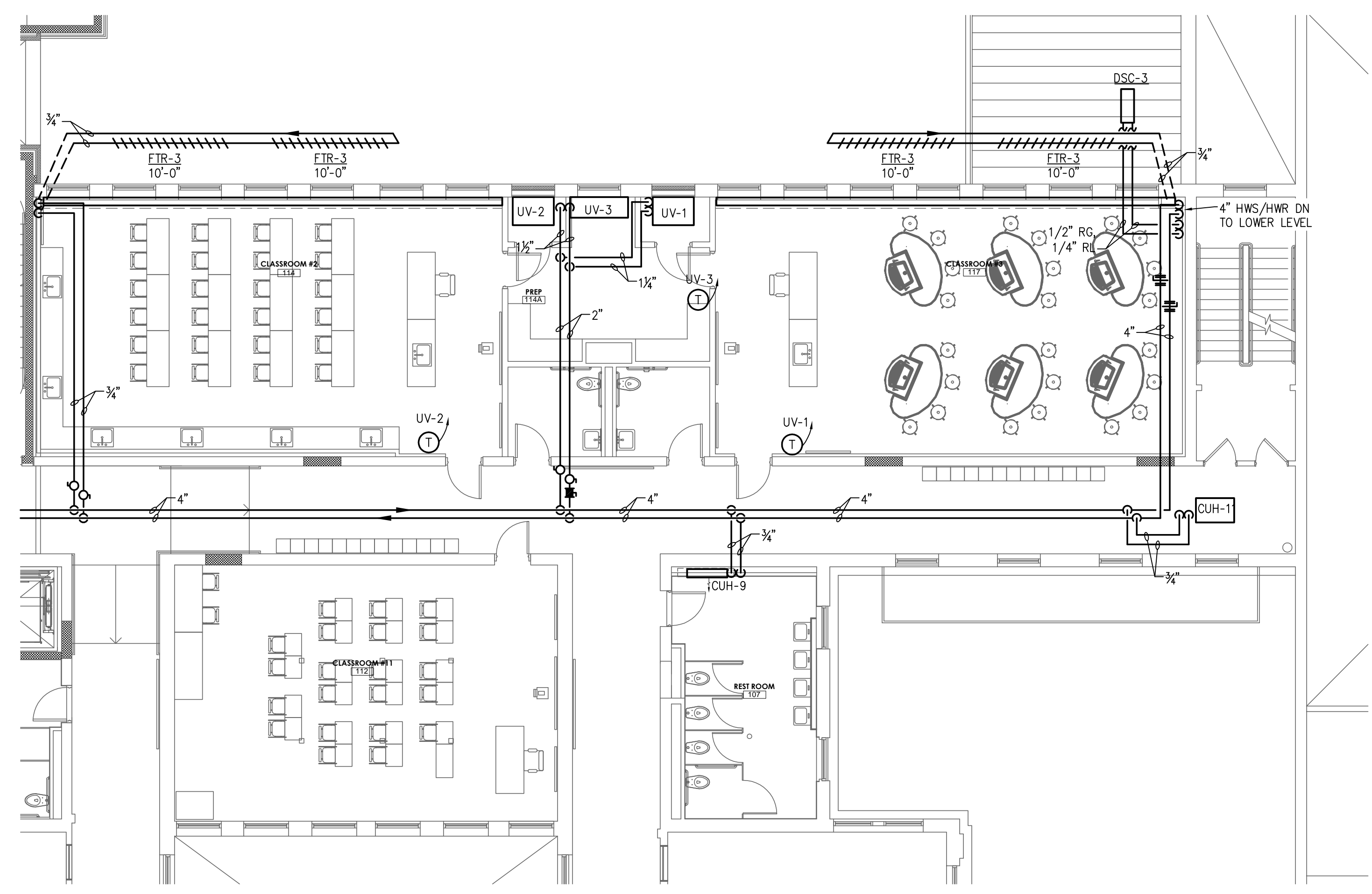
1 HVAC FIRST FLOOR PIPING PLAN H2.05 1/8" = 1'-0"
