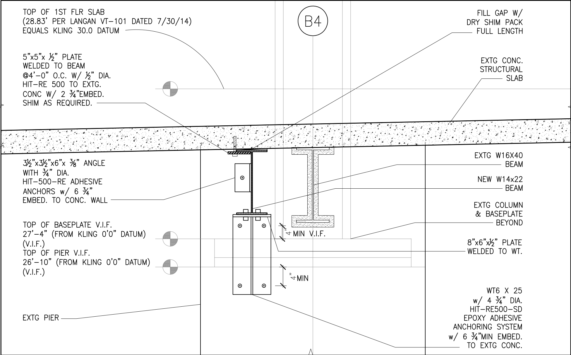
W14X22 BEAM SEAT AT B4 PIER
